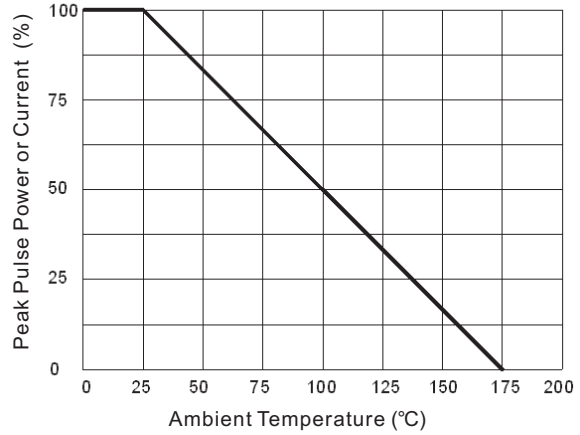
FIG 2-Pulse Power or Current VS Initial junction Temperature
