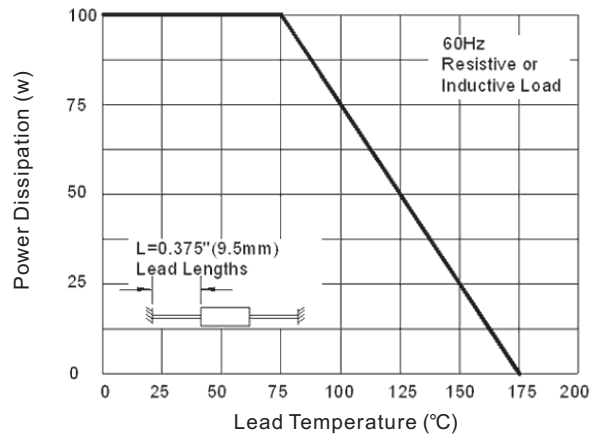
FIG 4-Power Derating Curve
