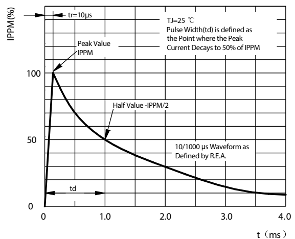
FIG2: Pulse Waveform
