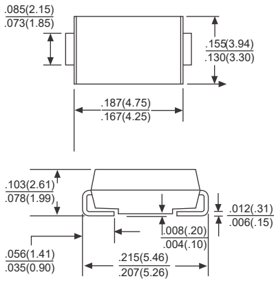
DO-214AA (SMB)
