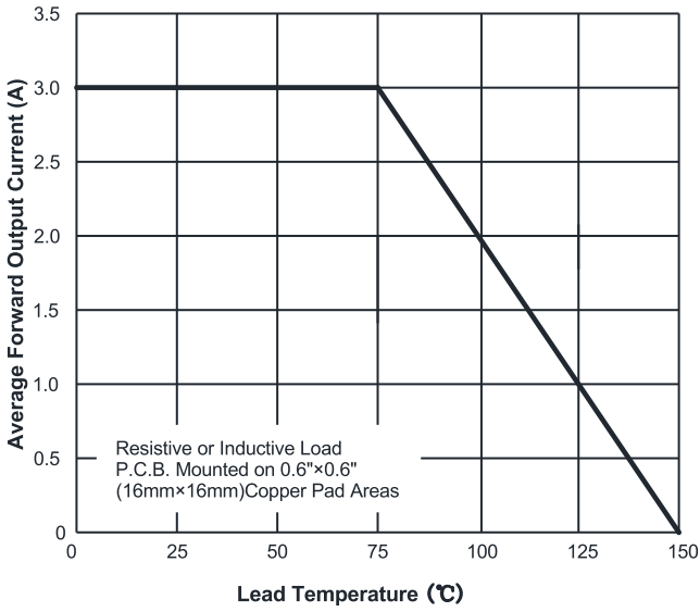
FIG.1: Io-TL Curve
